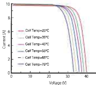
Current-Voltage Curve (LR6-60HPH-310M)
