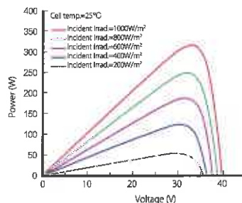
Power-Voltage Curve (LR6-60HPH-310M)
