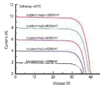
Current-Voltage Curve (LR6-60HPH-310M)
